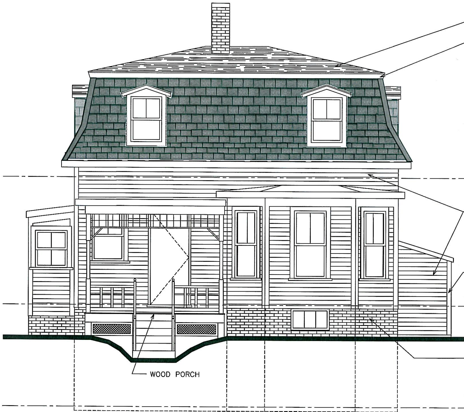
MANSARD ELEVATION WITH PROPOSED GAF DESIGNER "SLATELINE" SHINGLE (CUT SHEET ATTACHED)
